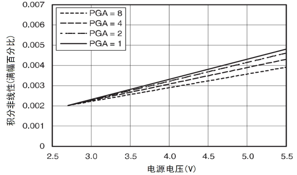
积分非线性 vs 电源电压
